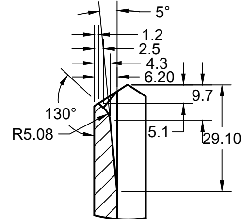
DETAIL C SCALE 1:1
